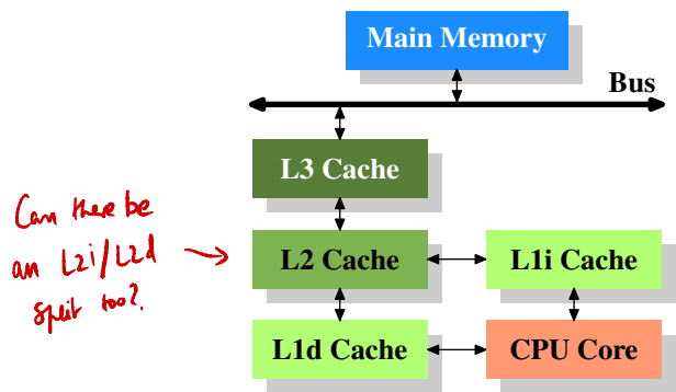
Figure 3.2: Processor with Level 3 Cache
