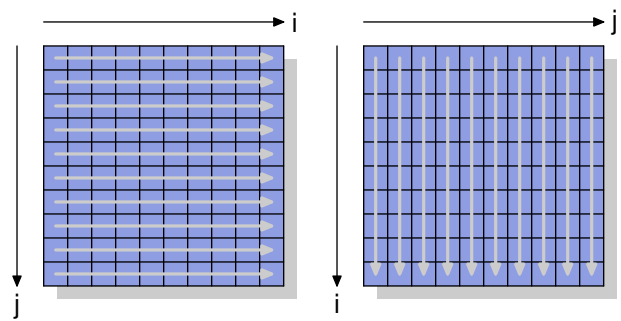
Figure 6.1: Matrix Access Pattern
