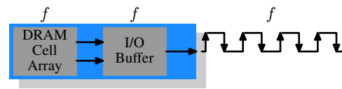
Figure 2.11: DDR1 SDRAM Operation
