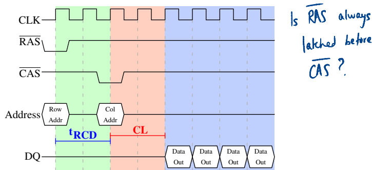
Figure 2.8: SDRAM Read Access Timing
